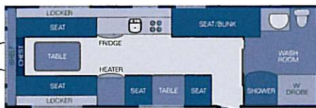
640-6 6 berth 6.4 metres
