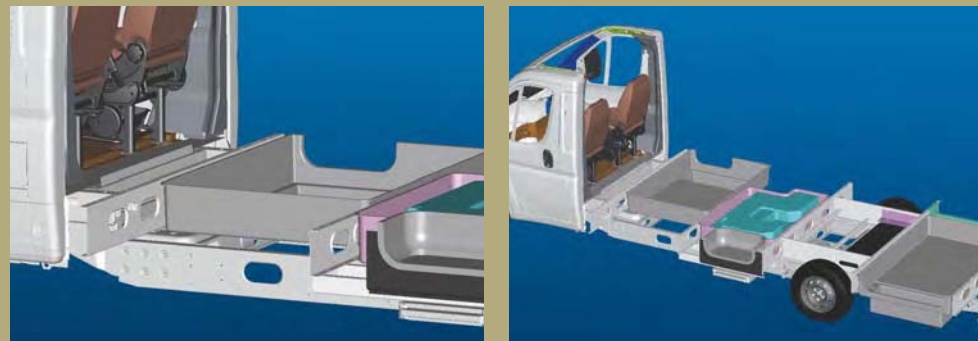
AL-KO double floor chassis houses the insulated fresh water tank, heating pipes and large storage trays
