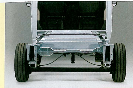
Wide track rear axle. (1)
