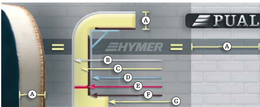
Unique Hymer-PUAL wall structure: Just 3.5 centimetres thick but the PUAL wall in the Hymermobil has the insulating effect of an 80 cm brick wall (A). The fine pored polyurethane foam (B) is joined completely to the sturdy aluminium outer skin (C) and the breathable plywood layer (D) inside the vehicle.
