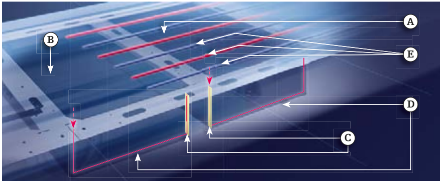
Insulated and heated underbody: The floor conceals the fresh water (A) and grey water tank (B) in insulated trays (C), which have hot air flowing through them (D).
