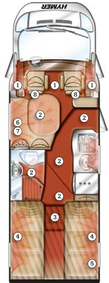
Pleasant even heat distribution: Many distributed hot air outlets guarantee perfect climate control. They also heat the water tank and the HVAC&S systems.
