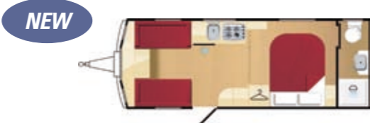
Supersirocco Twin Axle 4 berth
